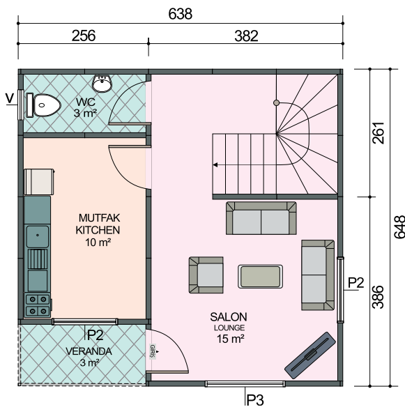
Zemin Kat Planı / Ground Floor Plan 38 m 2 + 3 m 2 = 41 m 2
