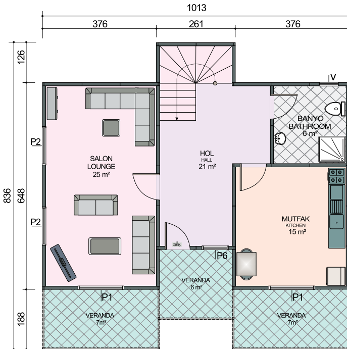
Zemin Kat Planı / Ground Floor Plan 66 m 2 + 20 m 2 = 86 m 2
