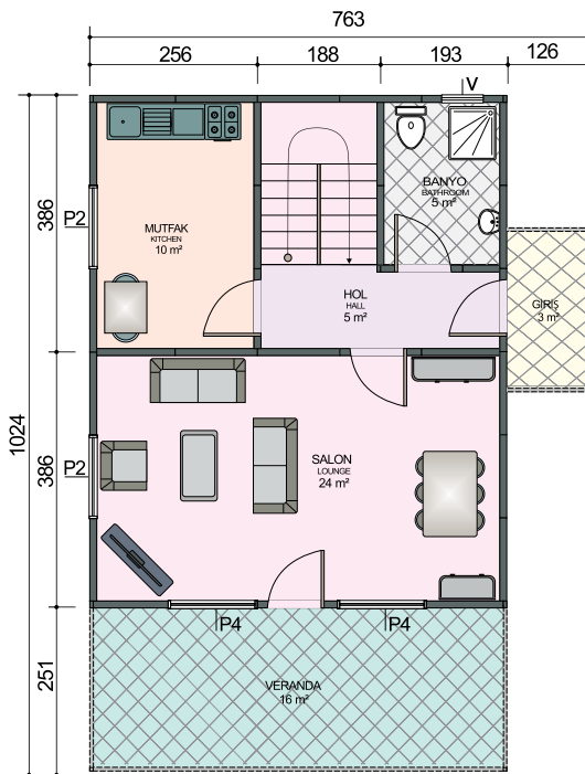
Zemin Kat Planı / Ground Floor Plan 49 m 2 + 16 m 2 = 65 m 2
