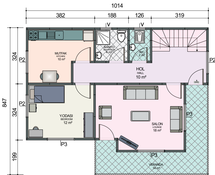
Zemin Kat Planı / Ground Floor Plan 64 m 2 + 14 m 2 = 78 m 2
