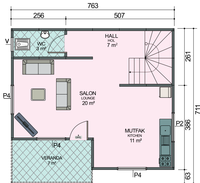
Zemin Kat Planı / Ground Floor Plan 45 m 2 + 7 m 2 = 52 m 2
