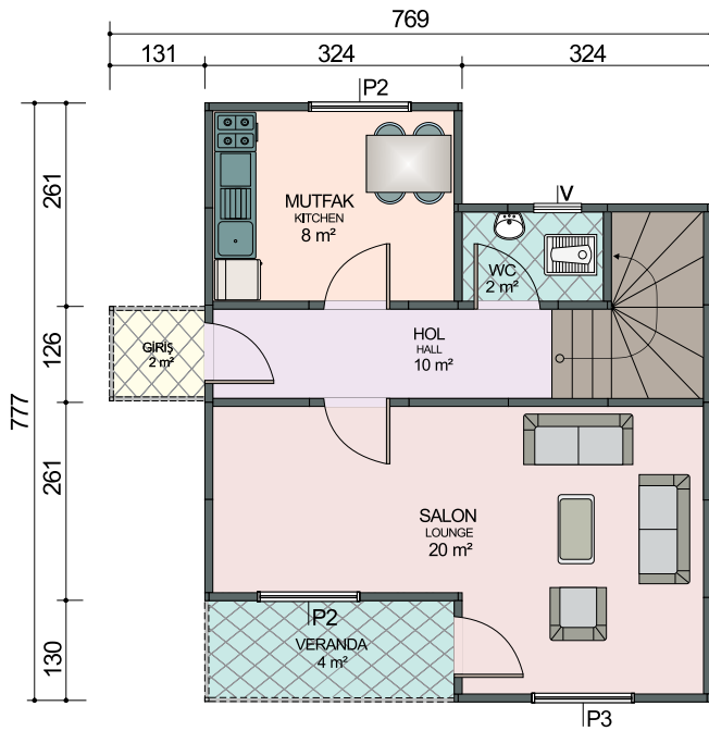
Zemin Kat Planı / Ground Floor Plan 41 m 2 + 6 m 2 = 47 m 2
