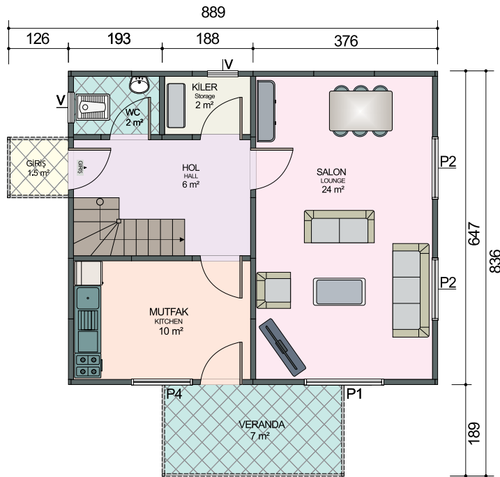
Zemin Kat Planı / Ground Floor Plan 49 m 2 + 9 m 2 = 58 m 2
