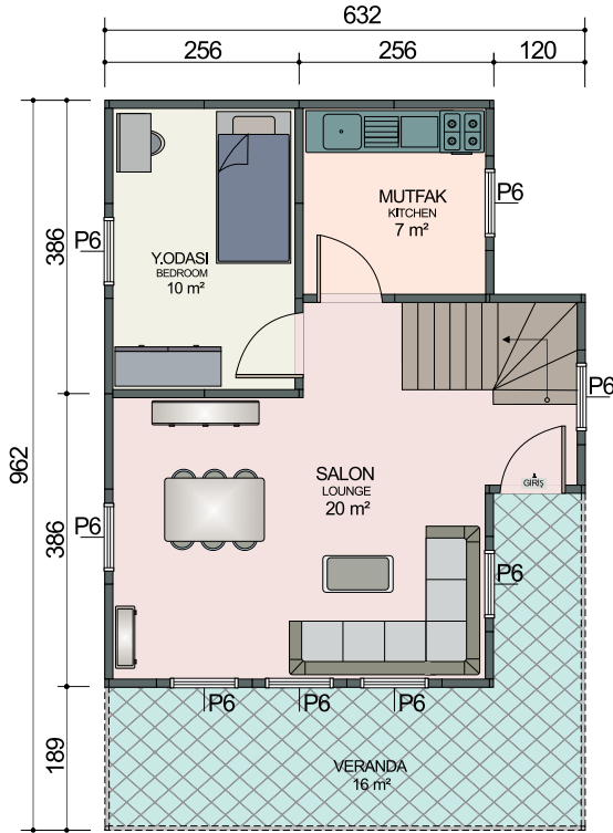
Zemin Kat Planı / Ground Floor Plan 42 m 2 + 16 m 2 = 58 m 2
