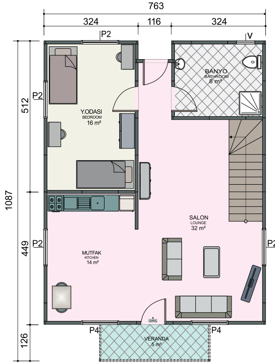
Zemin Kat Planı / Ground Floor Plan 74 m 2 + 5 m 2 = 79 m 2
