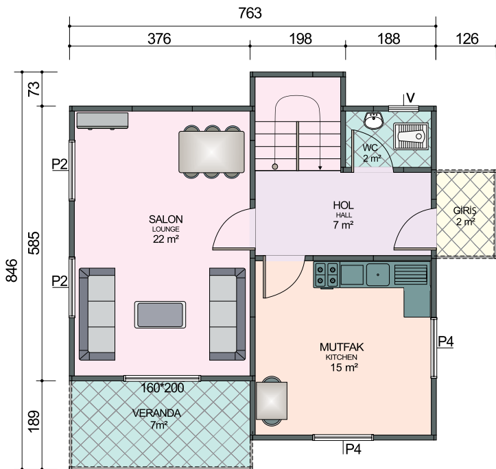
Zemin Kat Planı / Ground Floor Plan 51 m 2 + 9 m 2 = 60 m 2
