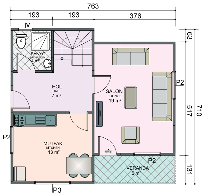
Zemin Kat Planı / Ground Floor Plan 46 m 2 + 5 m 2 = 51 m 2
